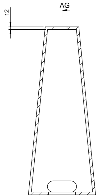
SECTION AF-AF
